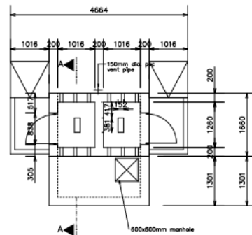
DOUBLE PIT LATRINE FLOOR PLAN
