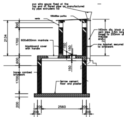
SECTION A-A FOR HIGH WATER TABLE
