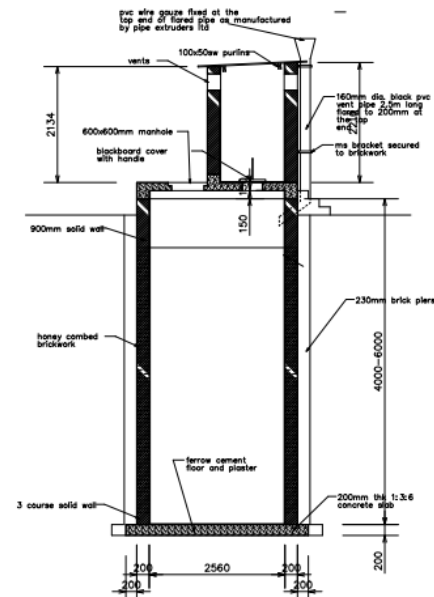
SECTION A-A FOR LOW WATER TABLE
